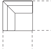
Angolo da 100x100 Corner element cm 100x100 L 100 P 100 H 75/93
