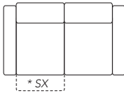
Divano 2 posti da 166 con 1 relax Dx/Sx 2 seater sofa cm 166 with 1 relax Rh/Lh L 166 P 101 H 81/99
