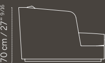
Fianco / Side
