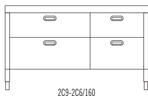
Elementi con cassetti 60-90 cm Elements with drawers 60-90 cm wide
